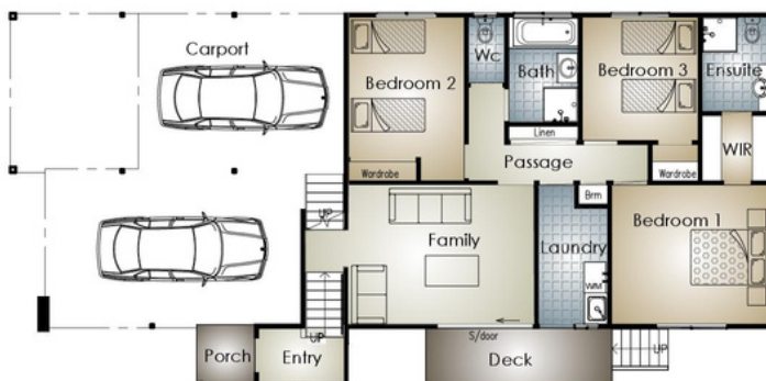
GROUND & MEZZANINE FLOOR
