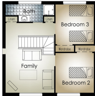
UPPER FLOOR PLAN
