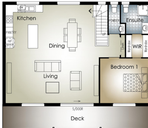
UPPER FLOOR
